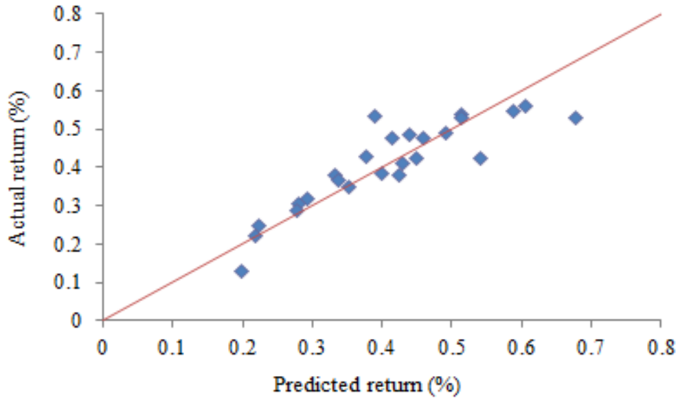
Panel A: 25-Size/Maturity-Sorted Portfolios of Corporate Bonds
