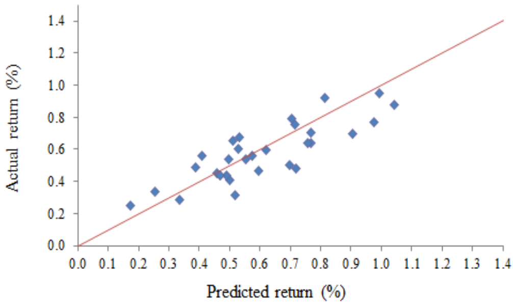
Panel B: 30-Industry-Sorted Portfolios of Corporate Bonds
