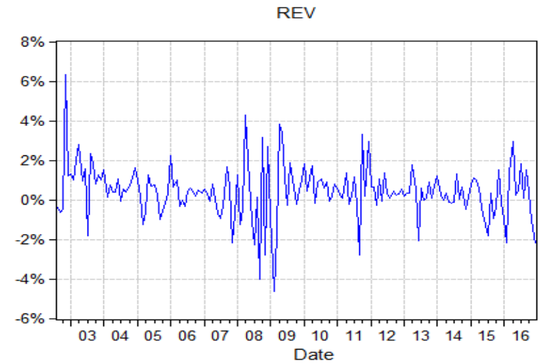
Fig.1. DRF, CRF, LRF, and REV Factors: 2002 – 2016. This figure plots the monthly time-series of the value-weighted downside risk factor (DRF), credit risk factor (CRF), liquidity risk factor (LRF), and return reversal factor (REV). DRF and CRF cover the period from July 2004 to December 2016. LRF and REV cover the period from August 2002 to December 2016.
