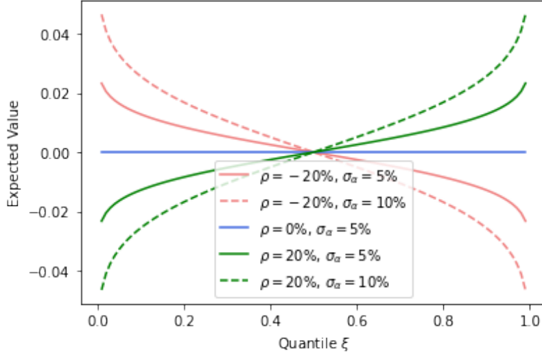
Figure 3: Asymptotic mean of the induced order statistic, \xi_{[i_k:N]} , as i_k \rightarrow N \xi \sim (0;1) .
